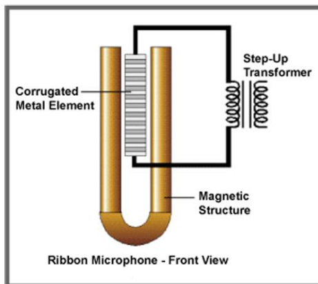
How a ribbon microphone works
