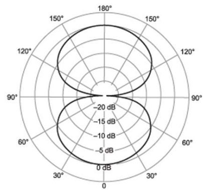
Bi-directional polar or pickup pattern
